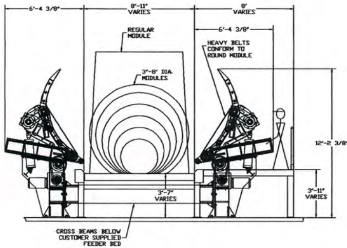
OPENED INFED END VIEW CONVEYS ROUND MODULE IN OR REGULAR MODULE THROUGH
