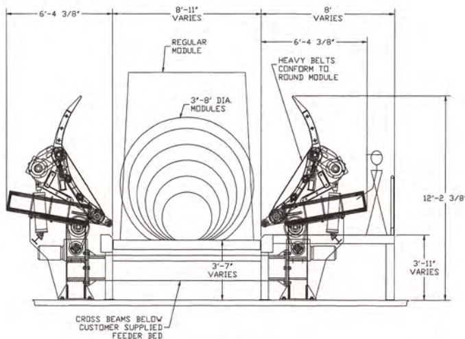
OPENED INFEED END VIEW CONVEYS ROUND MODULE IN OR REGULAR MODULE THROUGH
