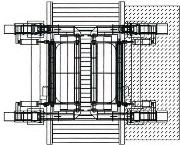
CLOSED TOP VIEW WITH MODULE LIFTED
