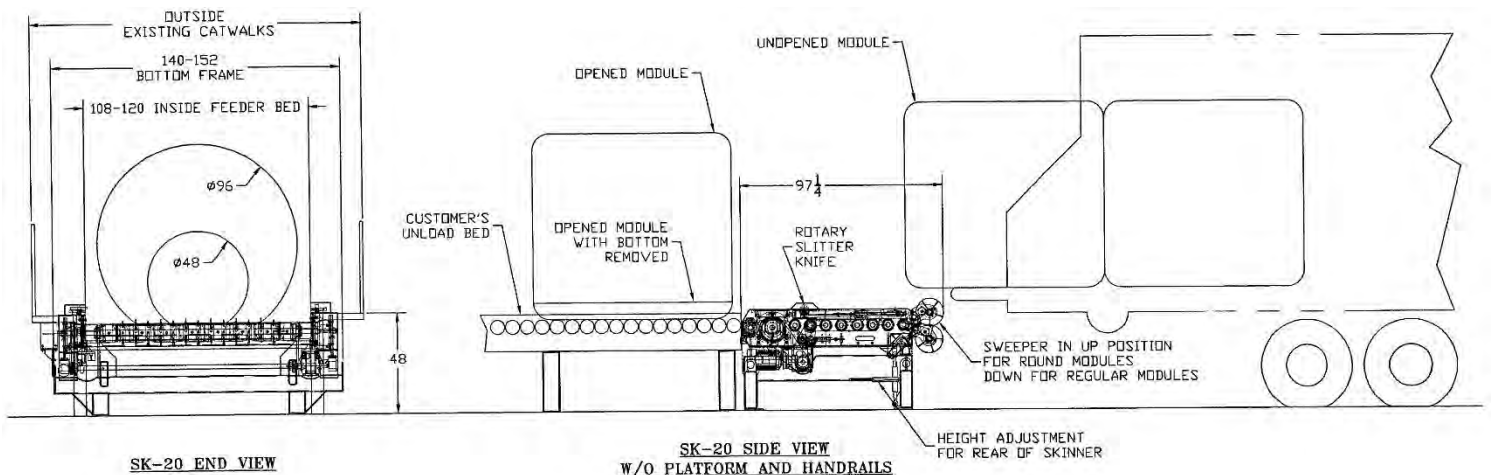
SK-20 END VIEW
