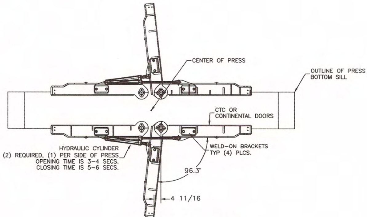
PLAN VIEW OPTION "B" USED WITH AUTOMATIC STRAPPERS REQUIRES 10 GPM PUMPING UNIT
